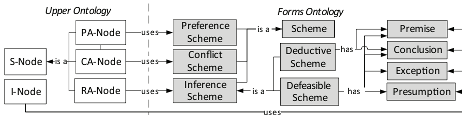
Figure 1. The Upper and Forms Ontologies of the AIF
