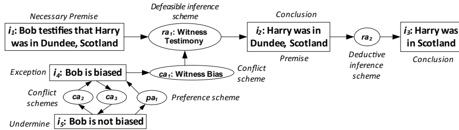
Figure 2. An AIF argument graph linked to the Forms Ontology
